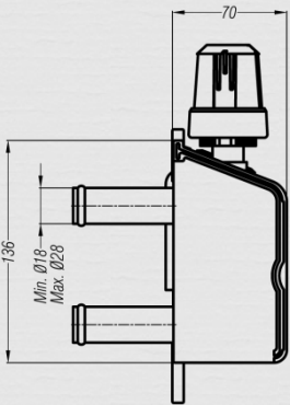
Convector Heater with Thermostatic Valve Termostatlı Konvektör
